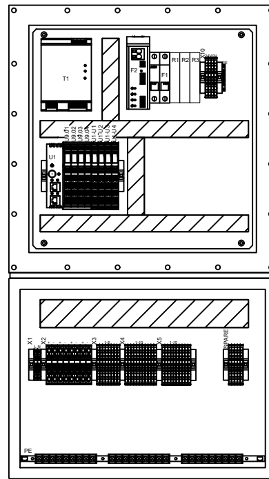
INTERNAL VIEW
