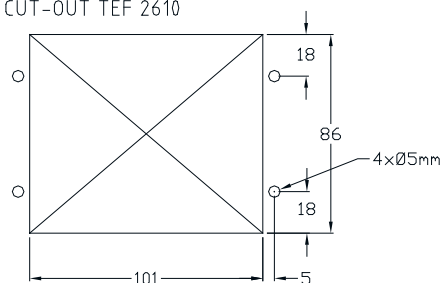
CUT-OUT TEF 2610
