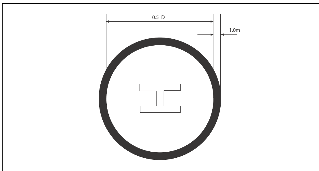
Figure 3 Touchdown/Positioning Marking Circle (TD/PM Circle to be painted yellow)
