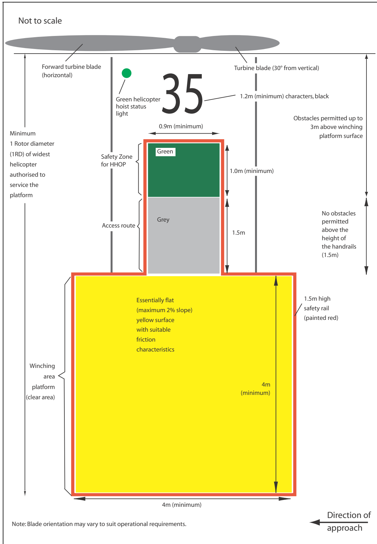
Figure 2 Winching Area, Access Route and Safety Zone
