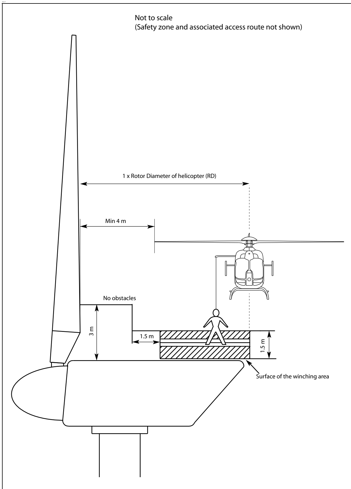
Figure 3 General Arrangement Drawing Showing Surfaces and Sectors
