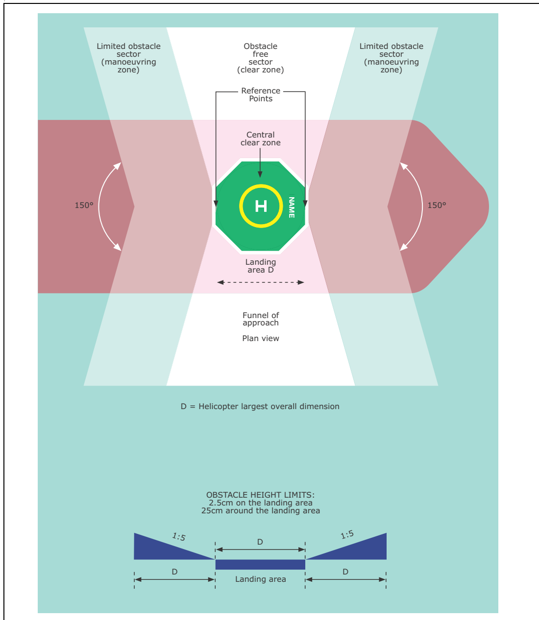
Figure 1 A Purpose-Built or Non-Purpose-Built Midship Centreline Landing Area 1
