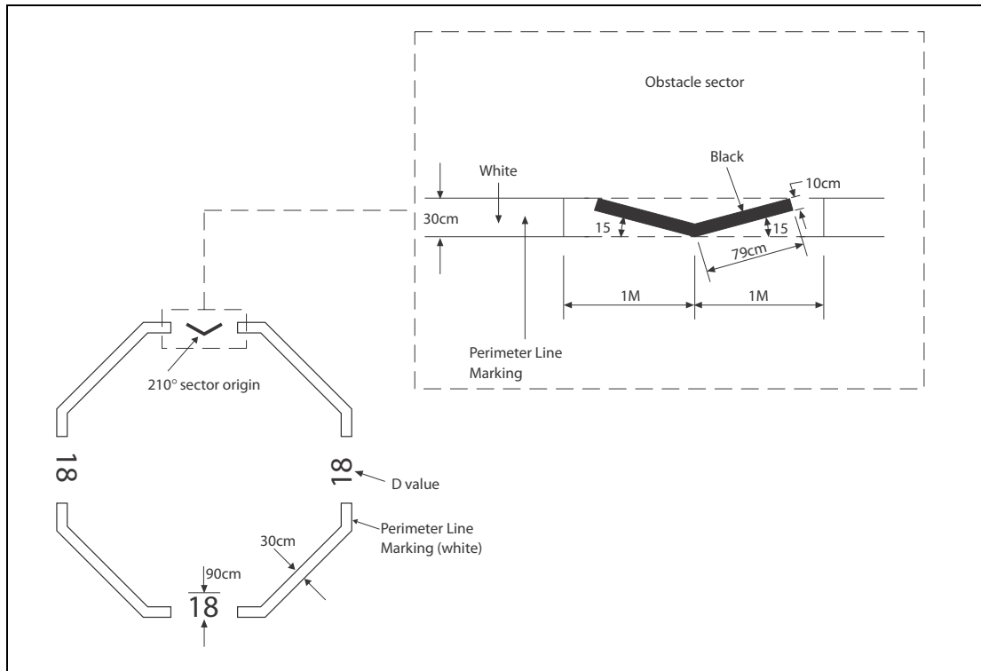
Figure 2 Helideck D-value and Obstacle-free Marking
